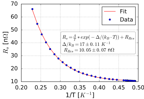
Figure 5: Surface resistance data fitting for cavity 001.
