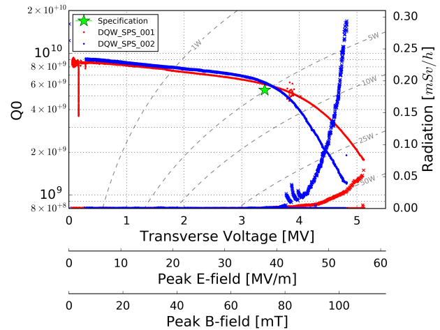
Figure 4: First performance results (at 1.9 K) for the DQW crab cavities to be installed the SPS test.
