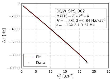
Figure 6: Lorentz Force Detuning data fitting for cavity 002.
