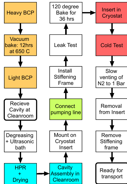
Figure 2: Schematic cavity preparation and testing sequence. The colour code of the activities is: Green = ISO5 environment, cyan = ISO4 environment, red = cryostat operation from 300K to 2K, orange = chemistry facility.
