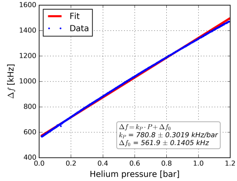
Figure 7: DQW_SPS_002 bare cavity with stiffening frame's pressure sensitivity for the 1.8 GHz mode.
