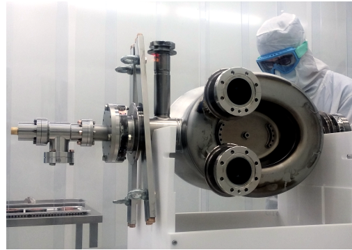
Figure 1: One of the two DQW_SPS crab cavities during clean room assembly (ISO4).
