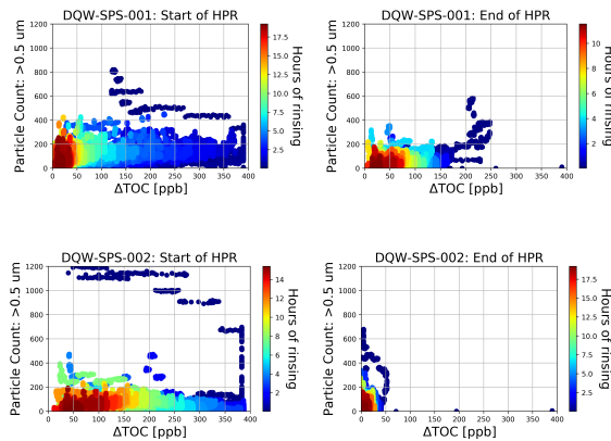
Figure 3: Water monitoring of the first and last rinses for both cavities.
